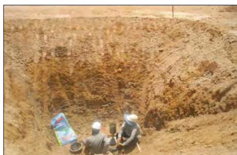
Field Density Testing
